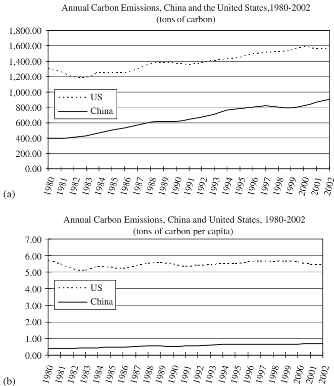
Fig. 1. (a) Annual carbon dioxide emissions from the consumption and flaring of fossil fuels, China and the United States, 1980–2002 (metric tons of carbon). (b) Annual carbon dioxide emissions per capita from the consumption and flaring of fossil fuels, China and the United States, 1980–2002 (metric tons of carbon per capita).
